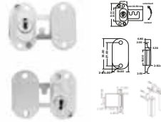
Aluminium Profile Lock For Double Door
