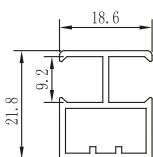
Aluminium Divider Profile
