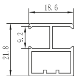
Aluminium Divider Profile
