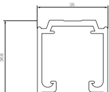
Top Track
