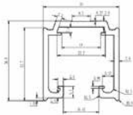
Top Track
