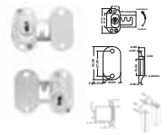
Aluminium Profile Lock For Double Door
