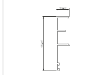
Aluminium Top Track Frame (Cover),
