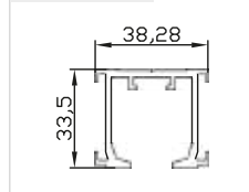
Top Track
