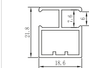
Aluminium Divider Profile
