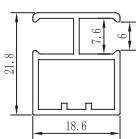
Aluminium Divider Profile
